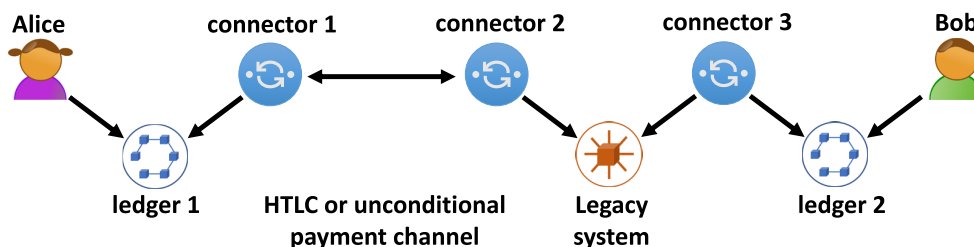
FIGURE 4. ILPv4 transaction between Alice and Bob with the help of three connectors. The connectors can use on-chain transactions, HTLC and unconditional payment channels, and legacy payment systems.
