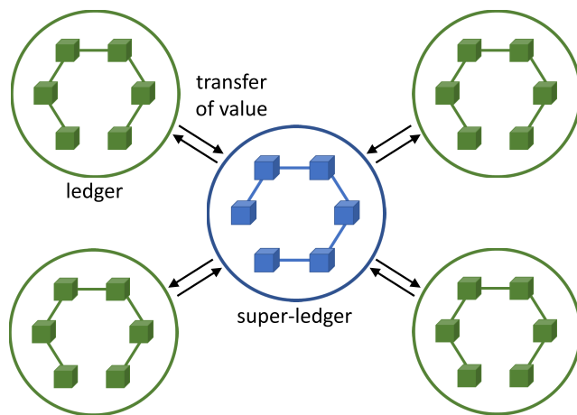
FIGURE 7. With the ledger-of-ledgers approaches a new super-ledger is introduced, which is the intermediary when two ledgers need to communicate.
