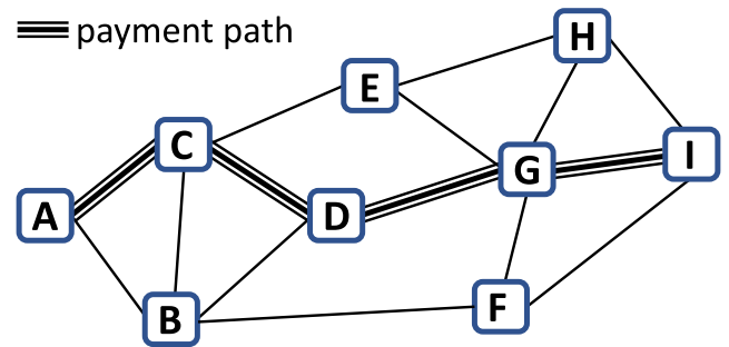
FIGURE 2. Nodes interconnected with a link are entities that have established a payment channel. In the Lightning network a payment path consists of a series of payment channels, which can involve different currencies of different blockchains.
