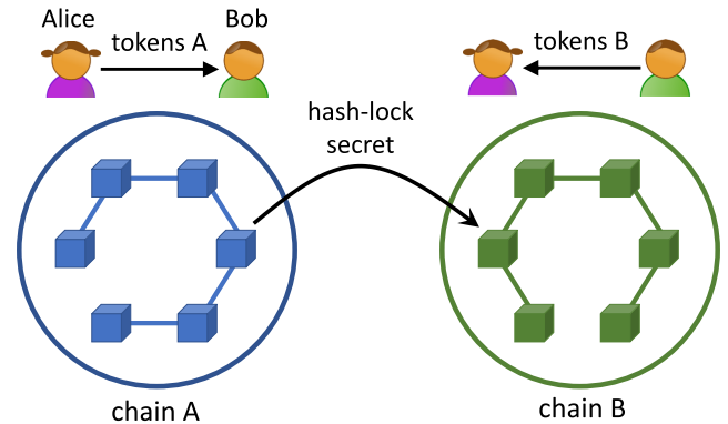
FIGURE 1. Atomic cross-chain trading. Having the same hash-lock value in the transactions on the two chains can ensure that either both of the two transactions (Alice and Bob exchanging tokens on the two blockchains) occur, once the hash-lock secret is revealed, or neither occurs.
