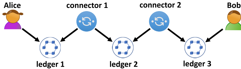
FIGURE 3. ILPv1 transaction between Alice (account in Ledger 1) and Bob (account in Ledger 3) via Ledger 2, with the help of two connectors.
